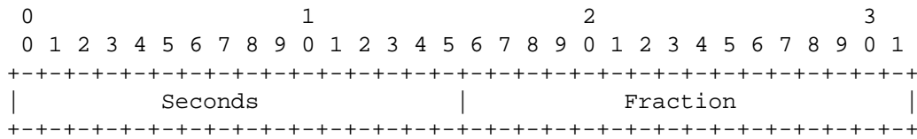
NTP Short Format
