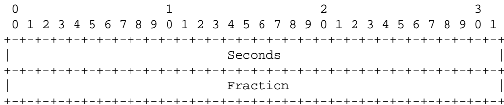
NTP Timestamp Format
